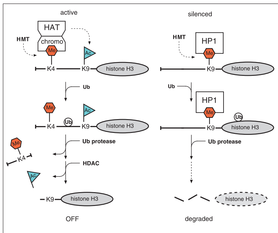
Fig. 3. A proteolytic model to remove “stable” methylation marks from histone H3. Abbreviations: Ub, ubiquitin-conjugating activity; Ub protease, ubiquitin-directed proteolytic activity. Depending on the chromatin environment and/or the nature of the ubiquitin signal, a methylated H3 NH 2 -terminus may be removed by proteolytic processing (left; see also Fig. 1D), or the entire H3 molecule may be degraded (right).
